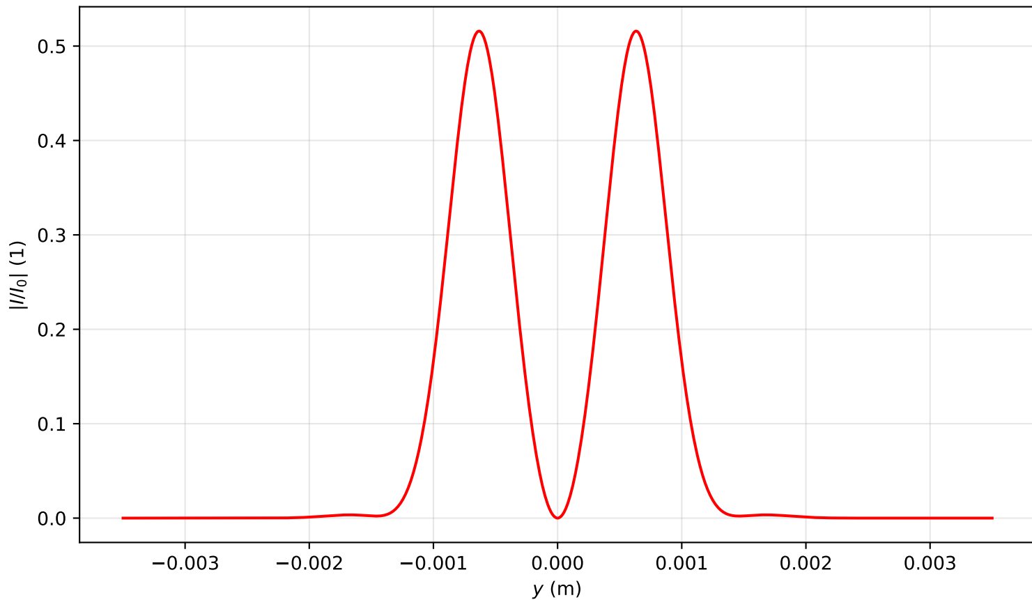
Intensity profile I(x=0, y, z=1.433)/I_0 , P_{in}=3.0P_{cr} , artificial time
